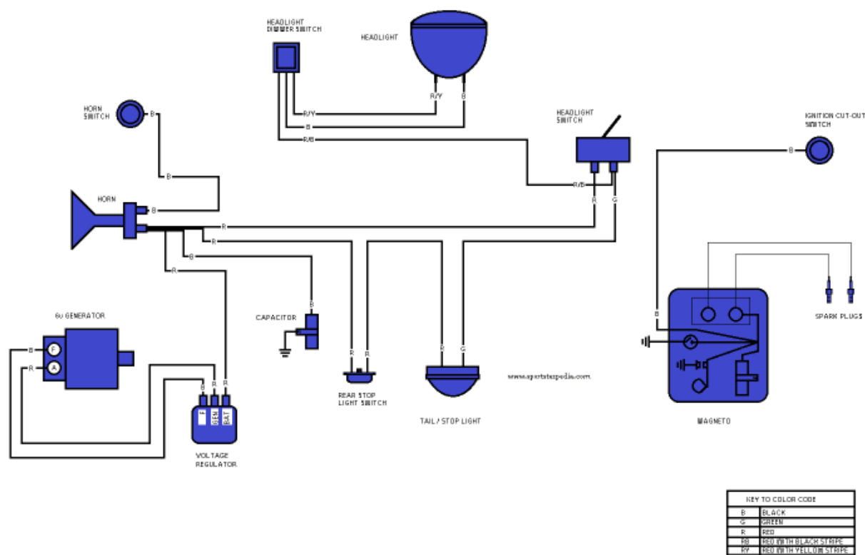
6v SYSTEM WIRING DIAGRAM
