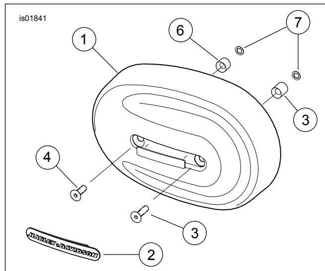
Figure 1. Service Parts: Air Cleaner Cover Kit
