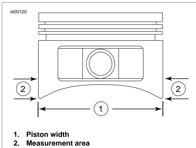
Figure 1. Piston Measurements
