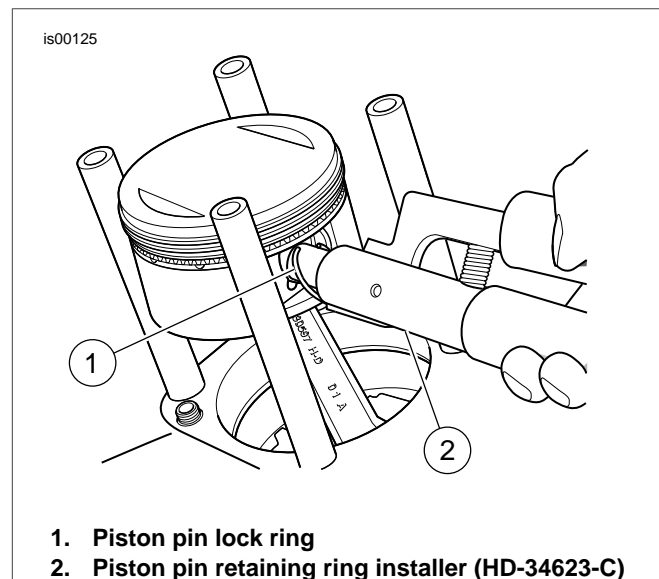
Figure 3. Seating Circlip
