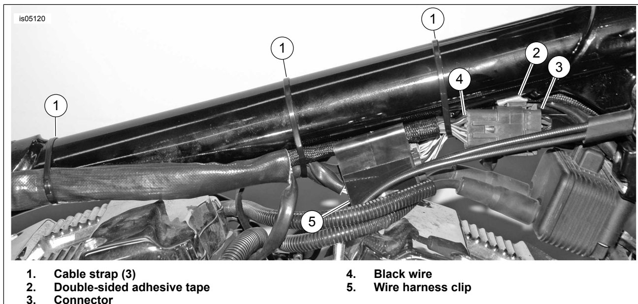
Figure 1. Harness Installation
